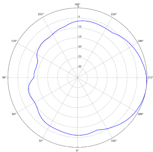
2.4GHz (Horizontal)
